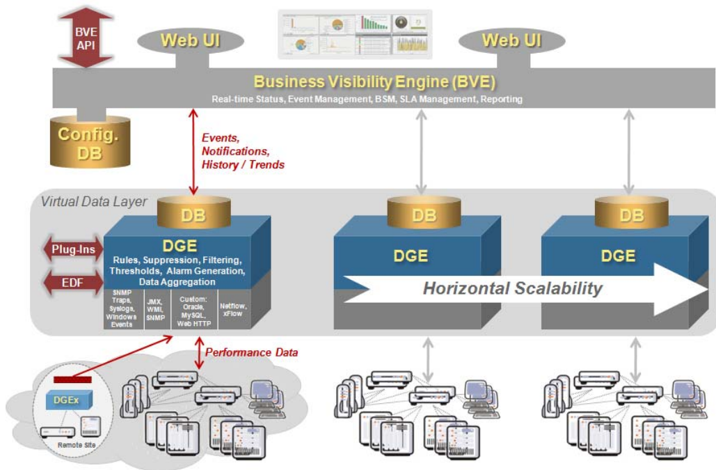
Fig 1: Enterprise and MSP Network Configuration
